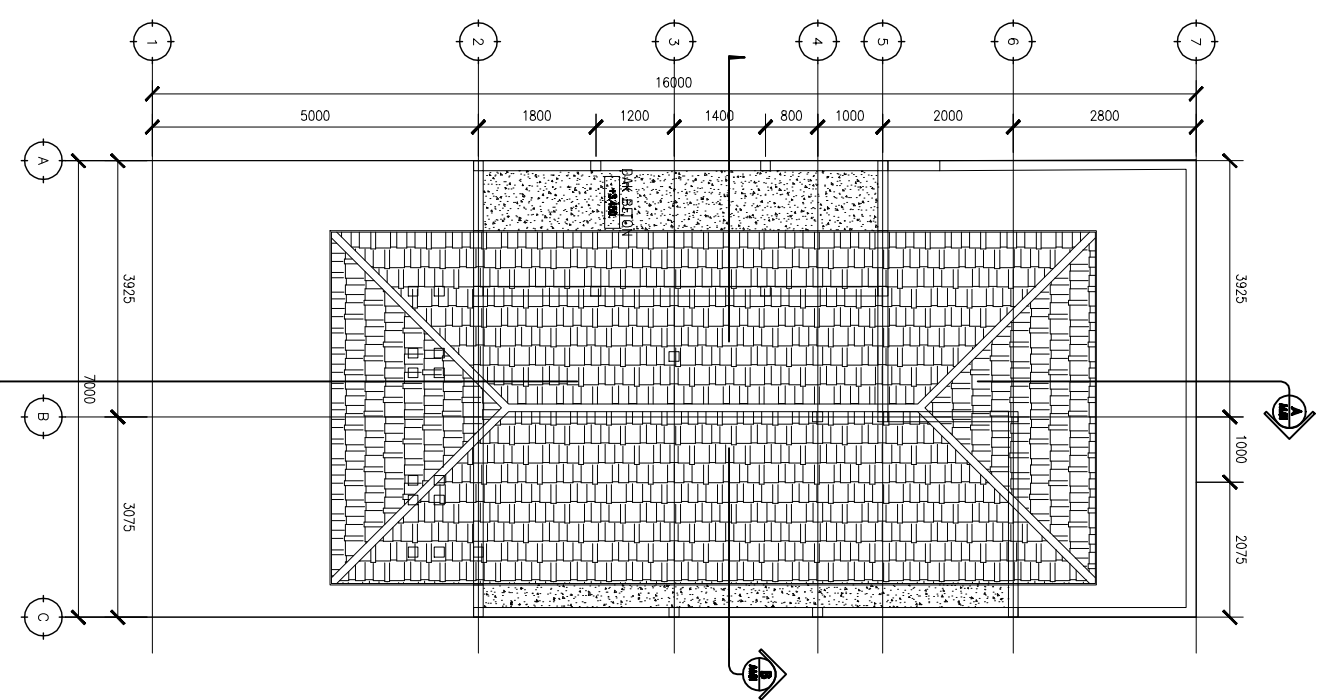
1 DENAH ATAP A2-1 1:100
